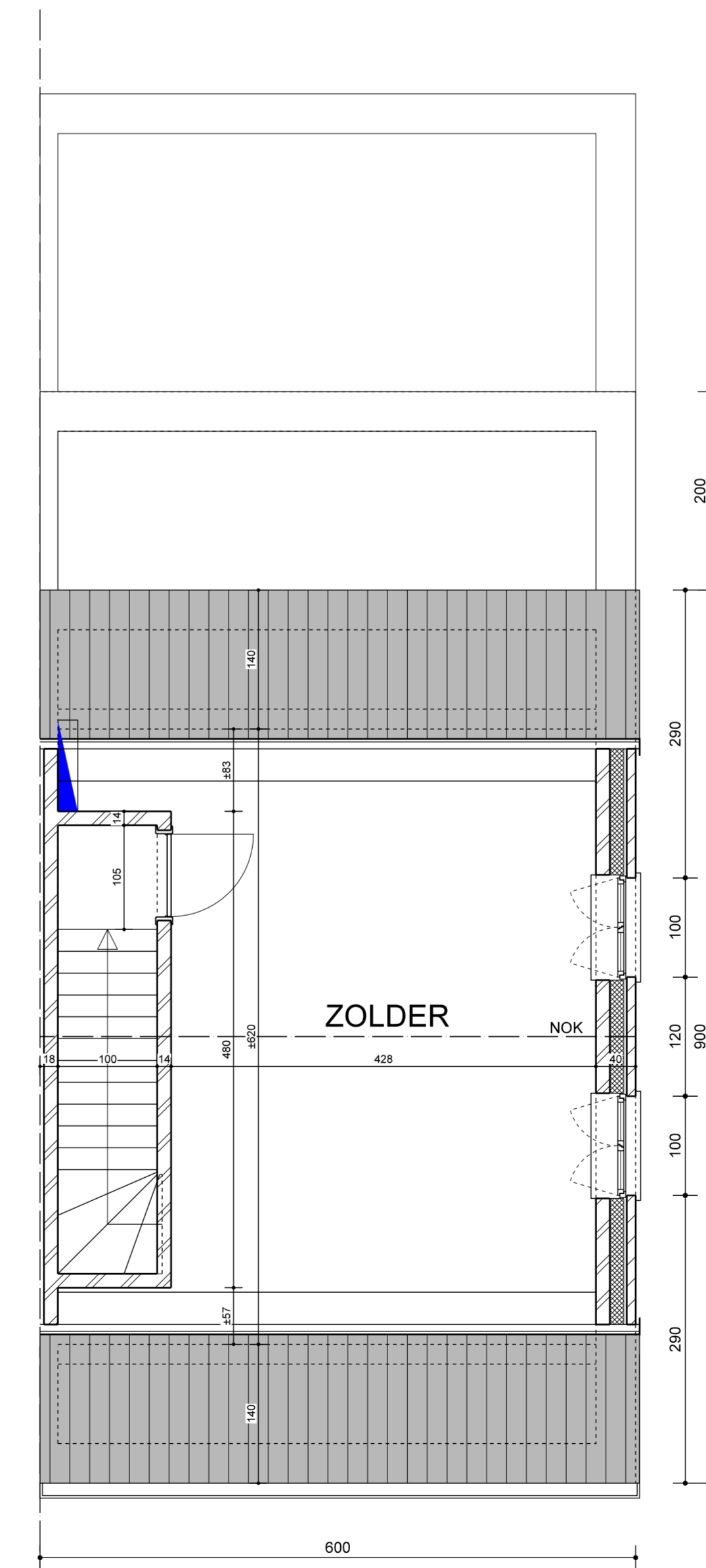
ZOLDER
